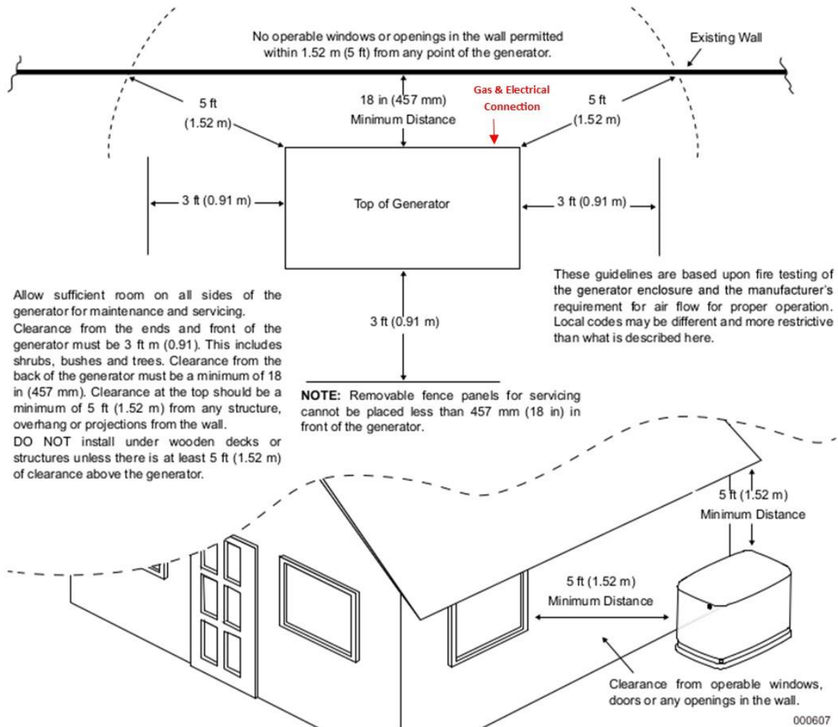
Figure 3-1. Installation Guidelines
